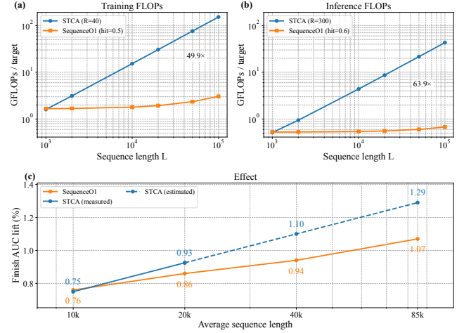
Figure 1: Compute-efficient scaling to 100K. (a) Training FLOPs of the ultra-long sequence branch for direct STCA and SequenceO1 from 1K to 100K under the observed training-side MRLB operating point ( R=40 , p_{\text{hit}}=0.5 ); at 100K, SequenceO1 is 49.9× cheaper than STCA. (b) Inference FLOPs of the same branch under the observed serving-side reuse operating point ( R=300 , p_{\text{hit}}=0.6 ); at 100K, SequenceO1 is 63.9× cheaper than STCA. Common recent-10K and ranker-side costs are omitted from both. (c) Finish AUC improvement over the STCA(512) baseline in the ablation setting versus average length; at 100K truncation (avg. 85K), SequenceO1 retains 83% of directly scaled STCA’s gain (+1.07% vs. +1.29%).
